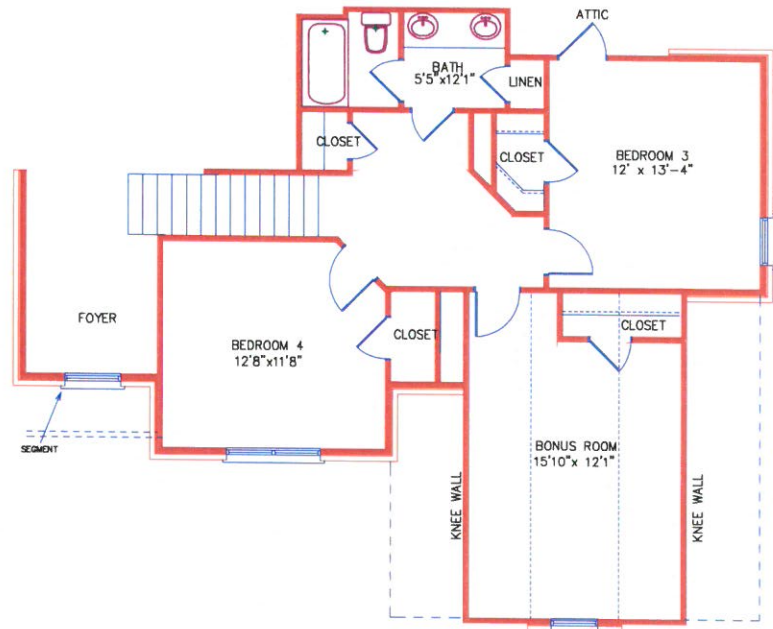
THE JACKSON SECOND FLOOR 820 S.F. HEATED
